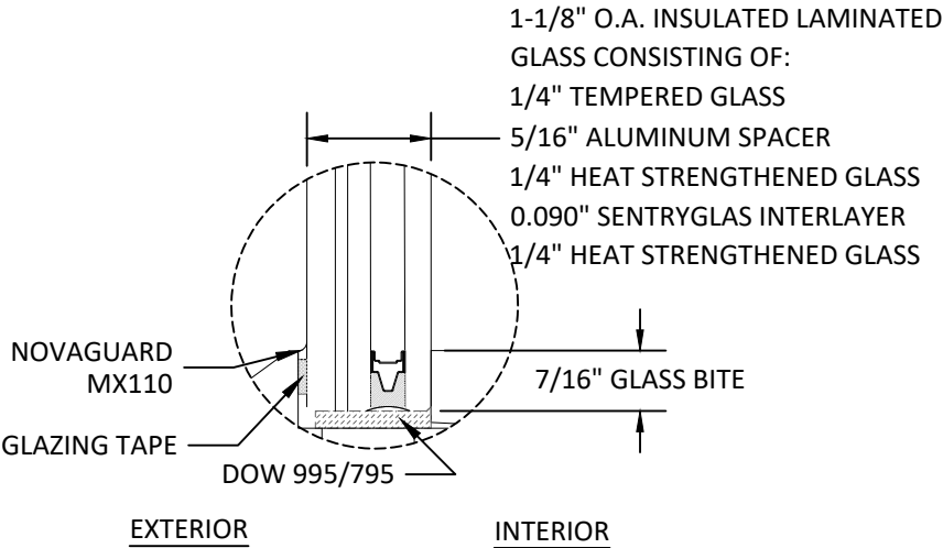
GLAZING DETAIL 2
