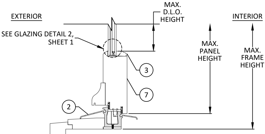
B 11 VERTICAL SECTION TYP. MIDRAIL DETAIL
