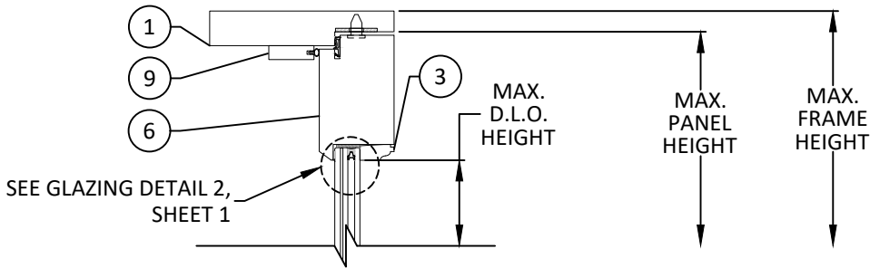
A 11 VERTICAL SECTION TYP. HEAD DETAIL
