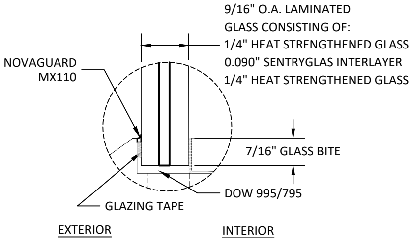
GLAZING DETAIL 1
