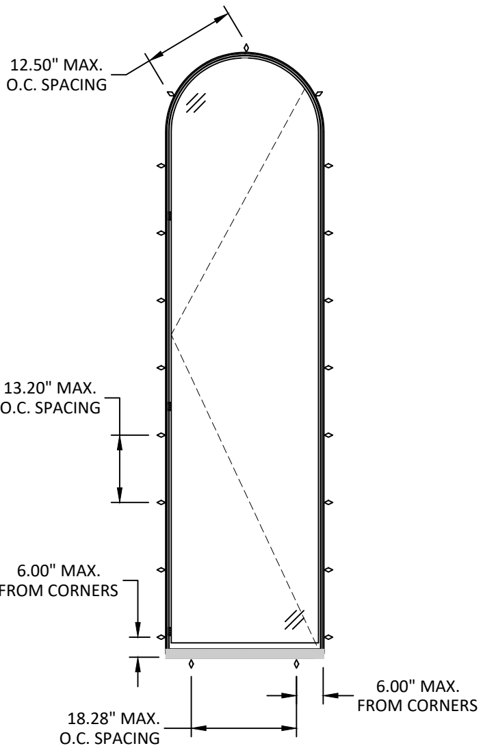
ANCHOR LAYOUT 16 GA. SIMPSON CS16Z STEEL STRAP / ALUMINUM ANGLE / Z-CLIP INSTALLATION
