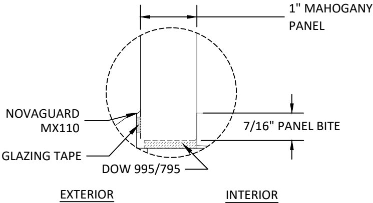
GLAZING DETAIL 3
