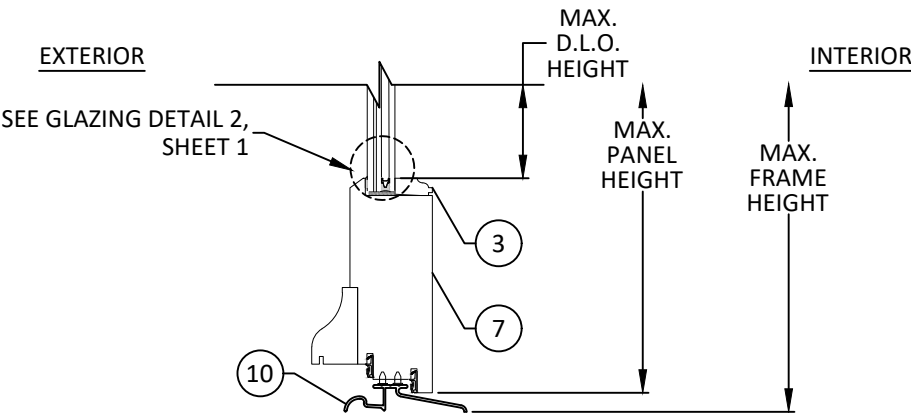
B 11 VERTICAL SECTION TYP. MIDRAIL DETAIL
